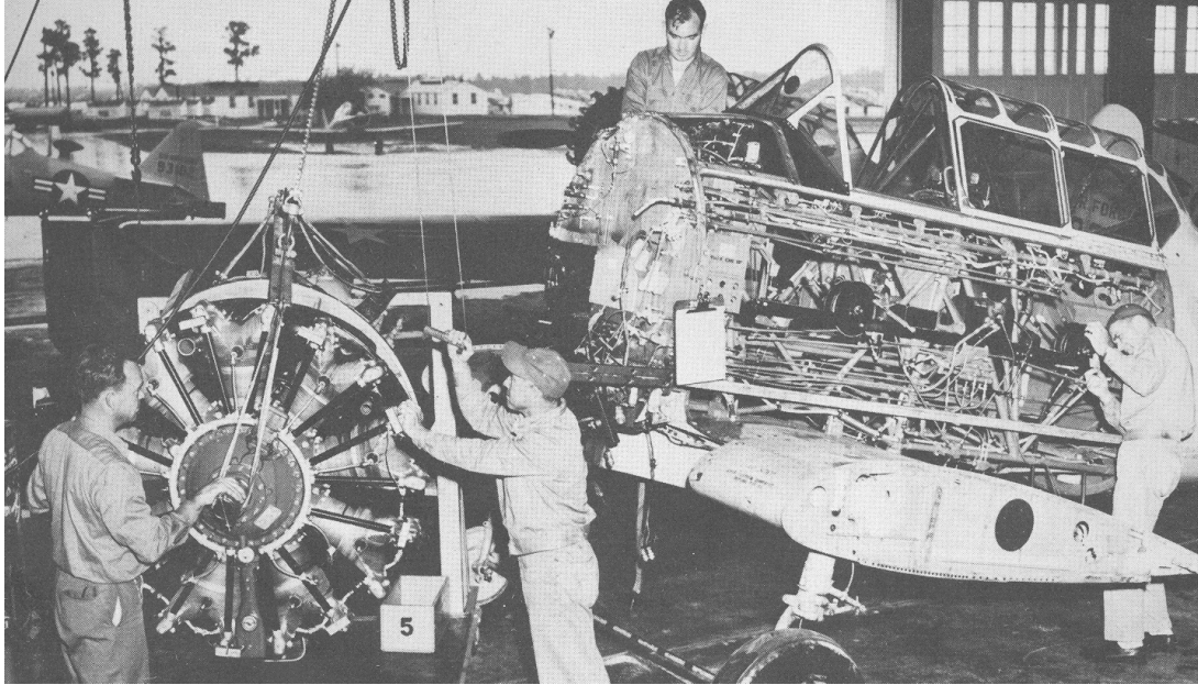
3303 Training Squadron (Contract Flying) T-6s undergoing maintenance. Bartow AB, FL, 1952. (USAF photo)
